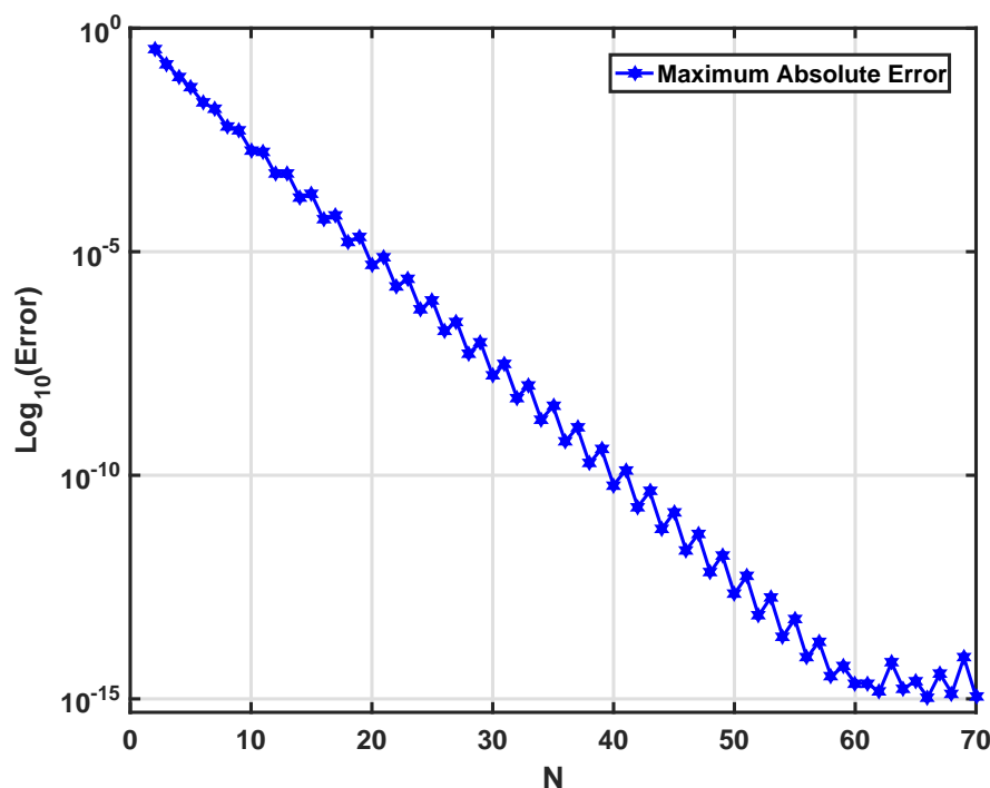
Figure 1: The maximum absolute error as a function of N for Example 1.
